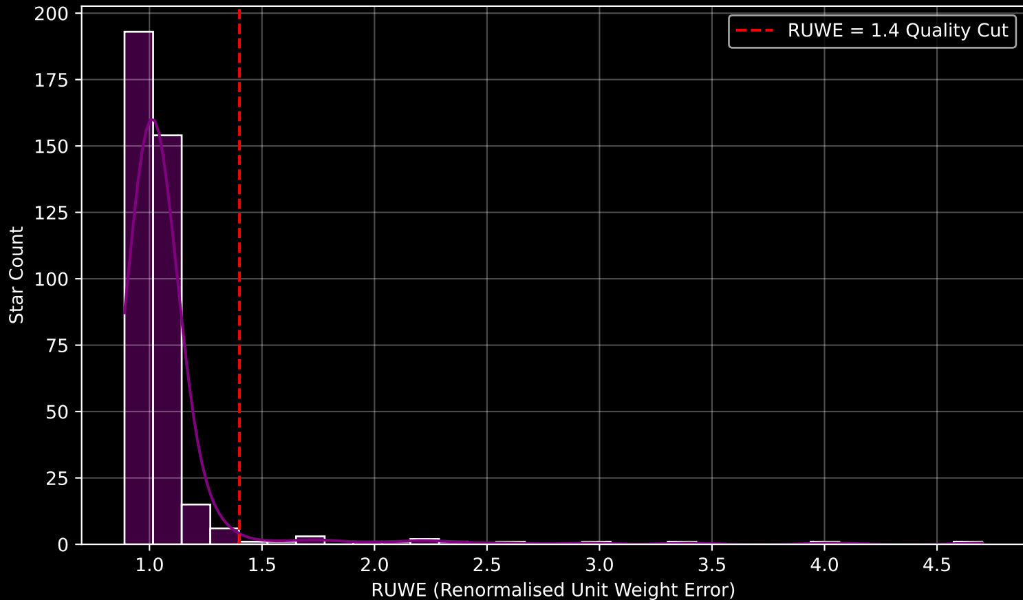
GAPOGEE DR17 Field [150+00] RUWE Distribution (n= 383)
