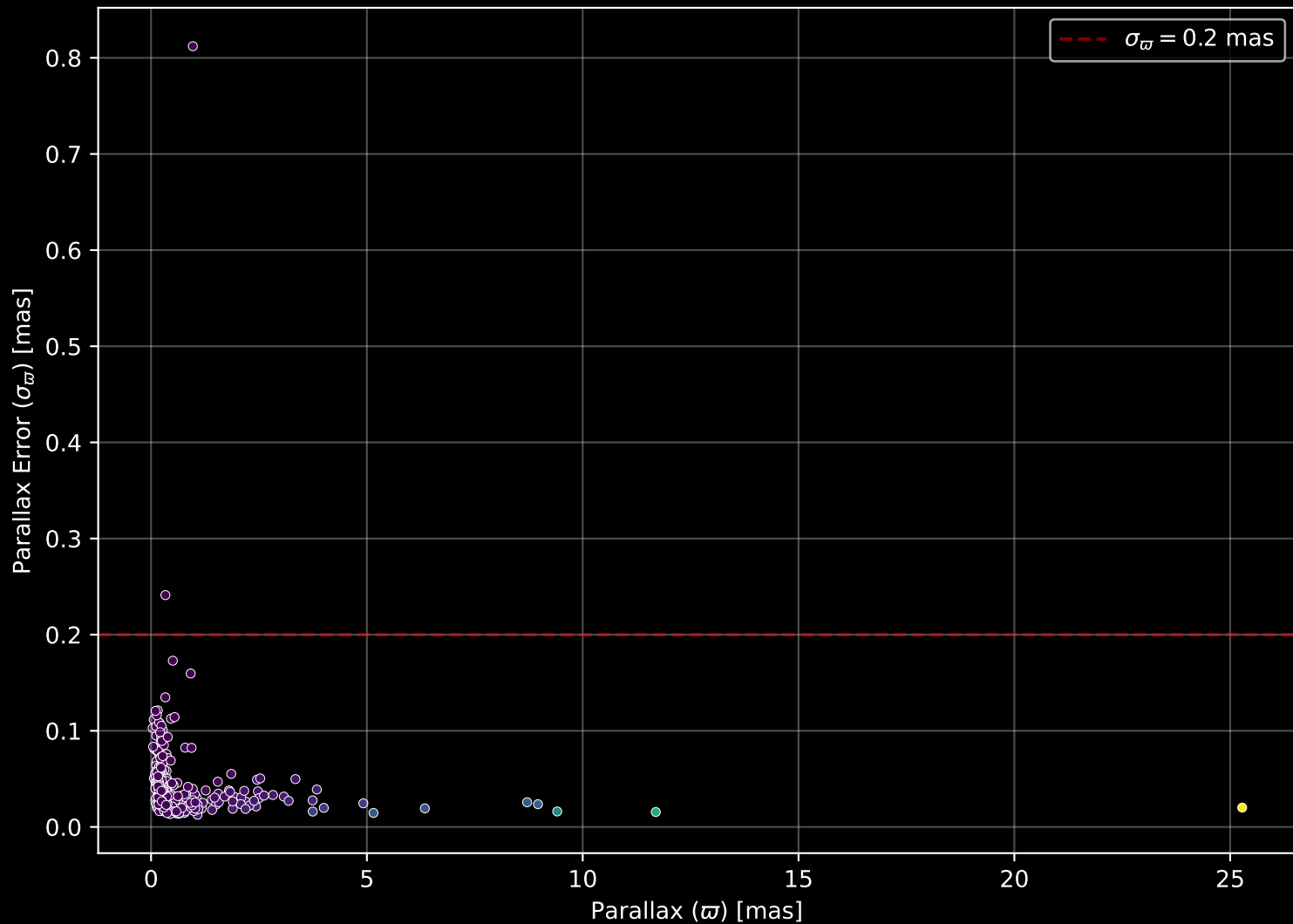
APOGEE DR17 Field: [150+00] Parallax Quality (n= 385)
