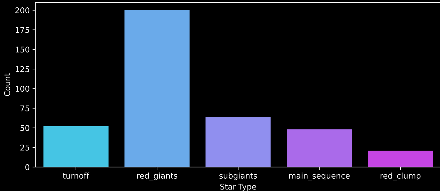
APOGEE DR17 Field: [150+00] Count plot of Star Type
