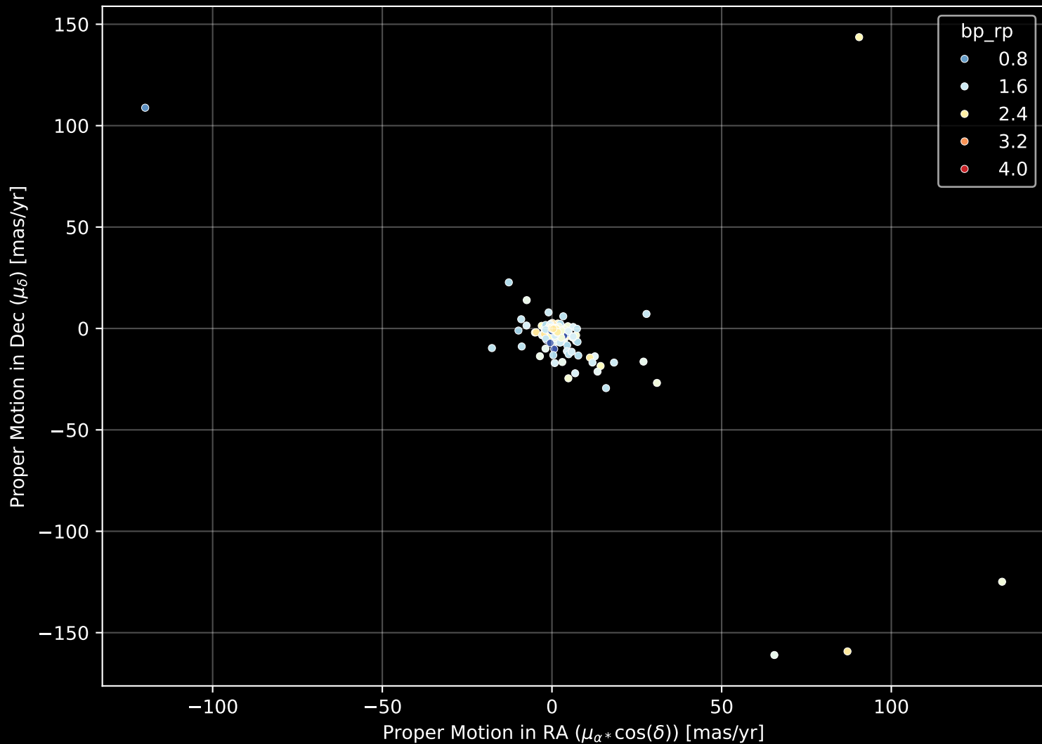
APOGEE DR17 Field: [150+00] Proper Motion Diagram (n= 385)
