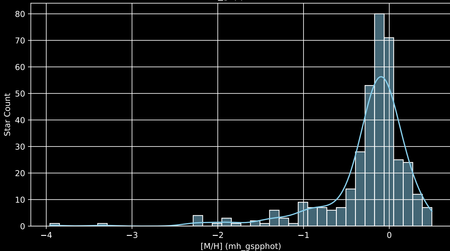
APOGEE DR17 Field: [150+00 [M/H] (mh_gspphot) (n= 374)
