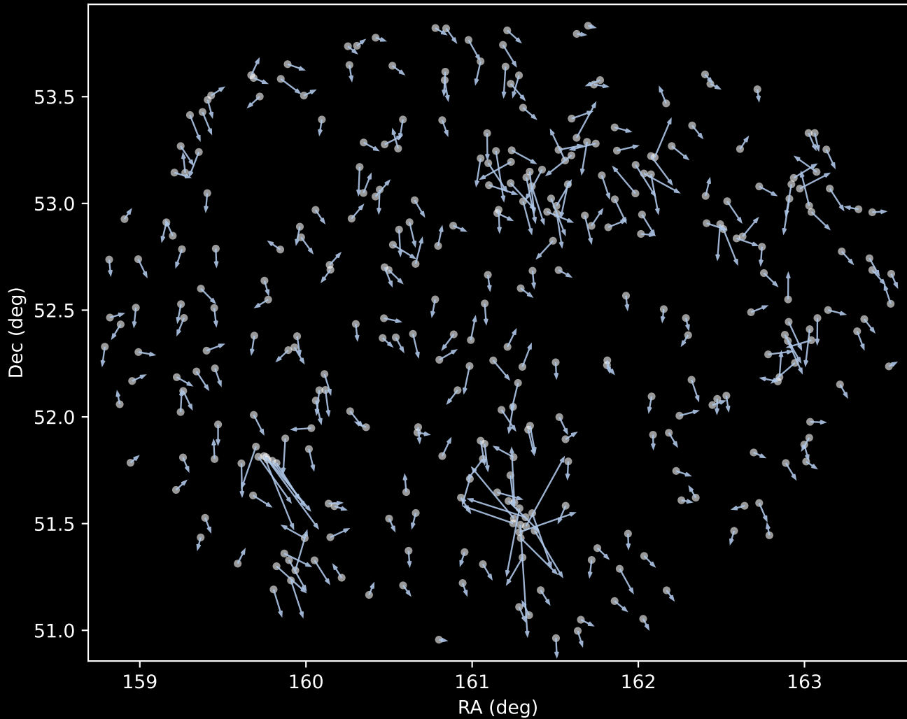
APOGEE DR17 Cluster 1 Proper Motion Vectors (n=330)
